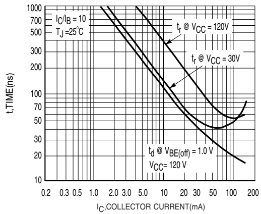
Figure 7. Turn-On Time
