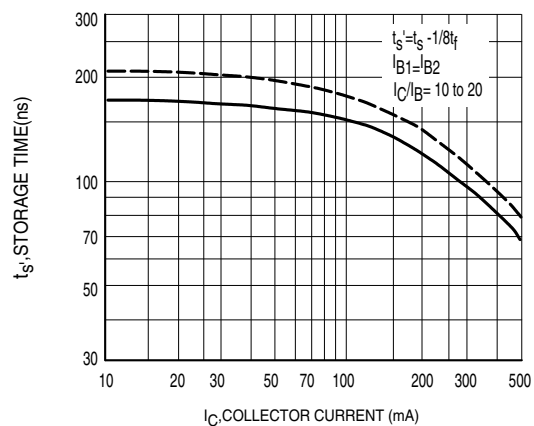
Figure 5. Storage Time
