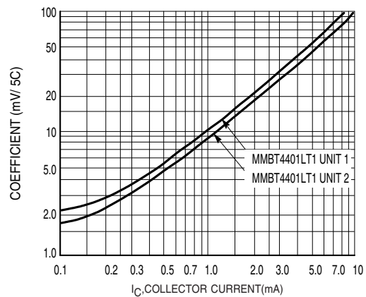
Figure 12. Temperature Coefficients
