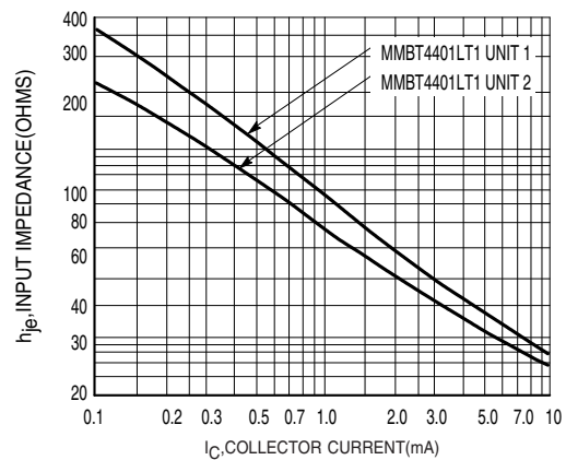
Figure 10. Input Impedance
