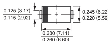
DO-214AB
