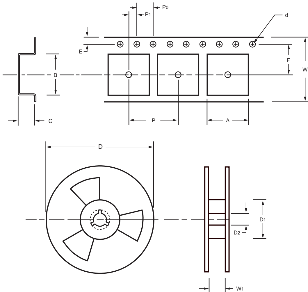
Fig.: Configuration of DIP REEL TAPING
