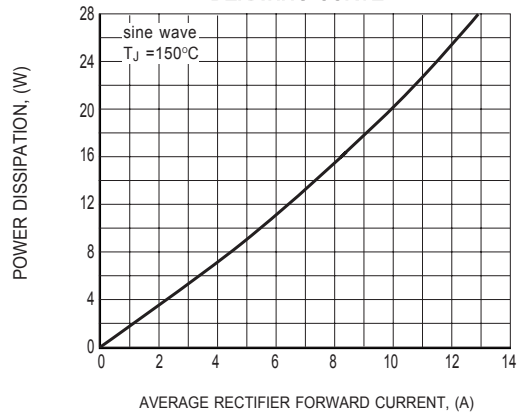
FIG.3 FORWARD DISSIPATION
